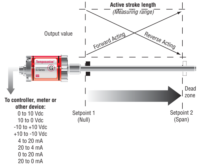
Figure 1. Single magnet analog output diagram
