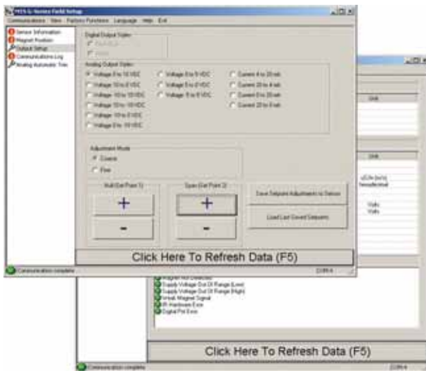
Figure 5. G-Series PC setup software interface examples
