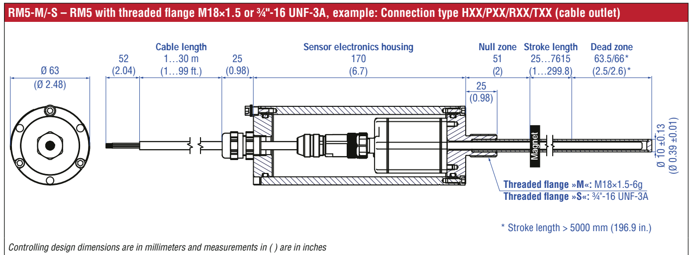
Fig. 2: Temposonics® RM5 with ring magnet
