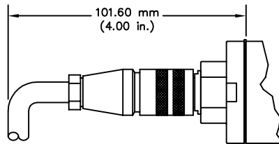
D6 Connector w/Straight Exit D6 Mating Connector
