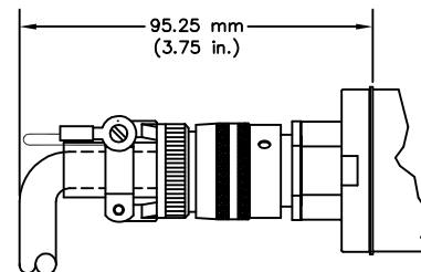
MS Connector w/MS Mating Connector
