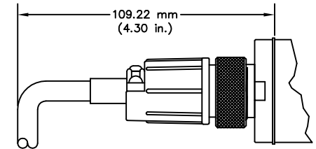
RB Connector w/MT or FT Mating Connector
