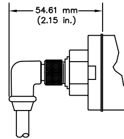
RG Connector w/90° RA Mating Connector
