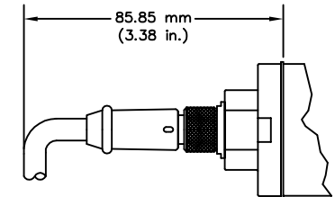
RG Connector w/Straight Exit RG Mating Connector
