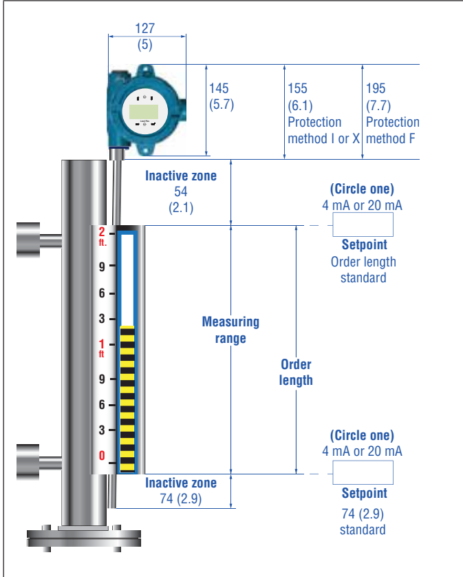
Fig. 3: CHAMBERED mounting, bottom flange 1
