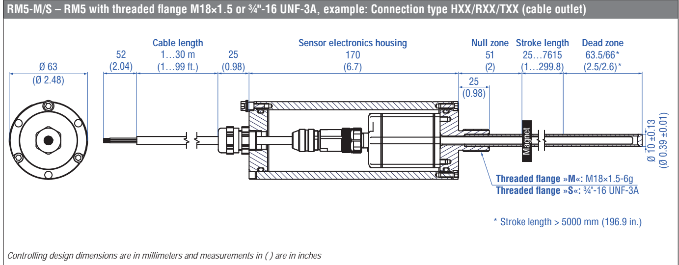
Fig. 12: Temposonics® RM5 with ring magnet
