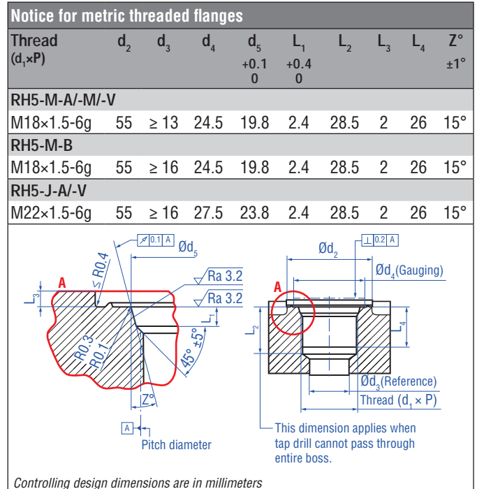
Fig. 11: Notice for metric threaded flange M18×1.5-6g/M22×1.5-6g based on DIN ISO 6149-1
