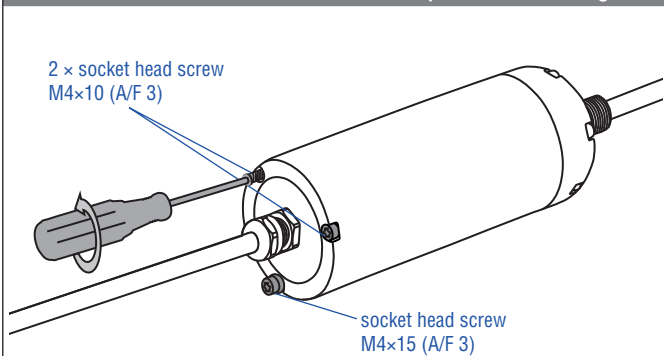
Fig. 54: Replacement of the base unit on model RM5, part 2
