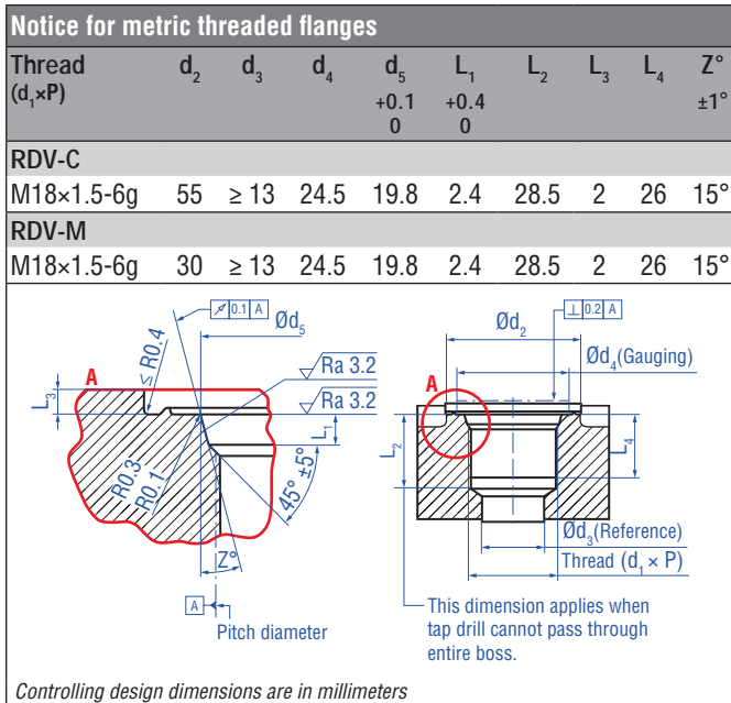
Fig. 30: Notice for metric threaded flange M18×1.5-6g based on DIN ISO 6149-1
