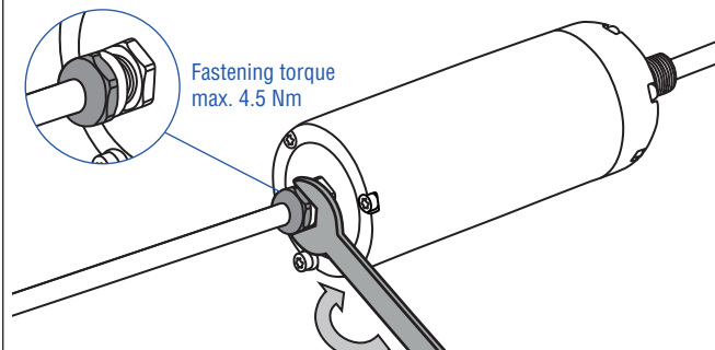
Fig. 56: Replacement of the base unit on model RM5, part 4
