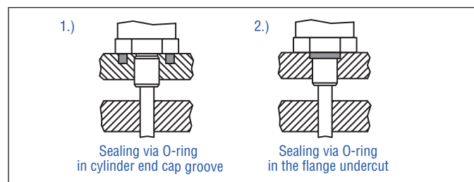
Fig. 23: Possibilities of sealing
