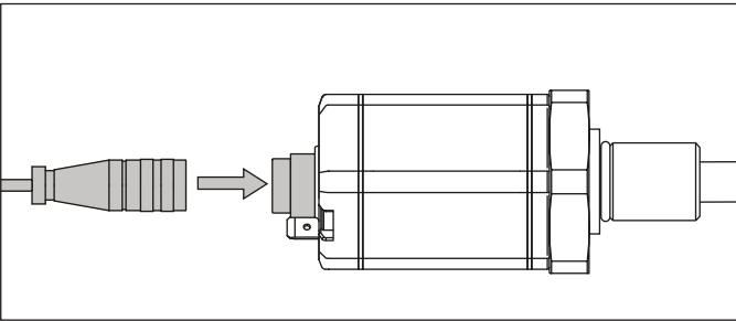
Fig. 70: Connection of adapter cable to R-Series V sensor with connector outlet
