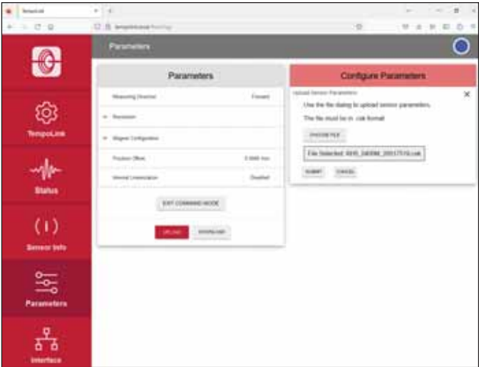
Fig. 83: Uploading a cek file to an R-Series V Analog sensor with the same stroke length
