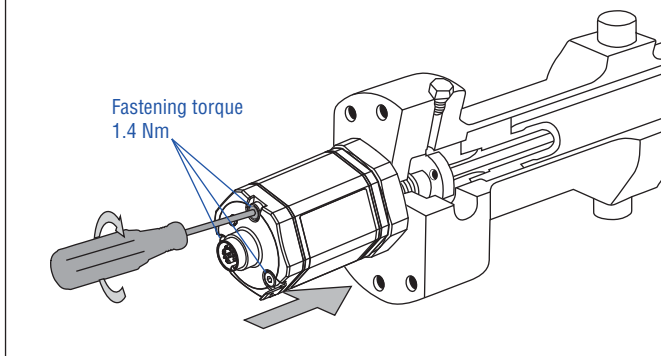
Fig. 51: Replacement of the base unit (e.g. RH5 sensor), part 2
