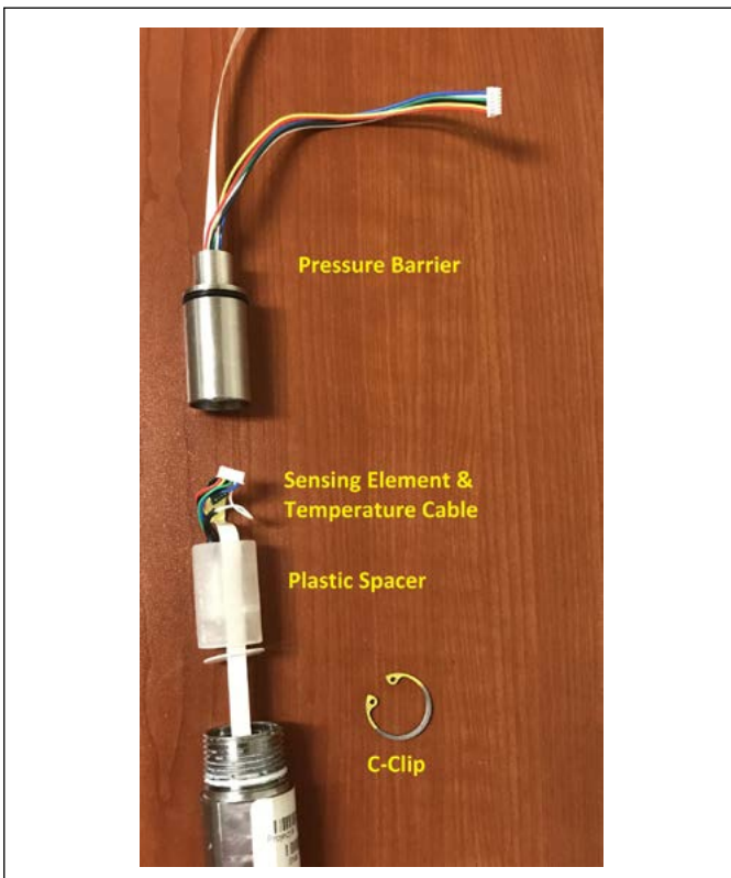
Fig. 11: Explosion proof cartridge
